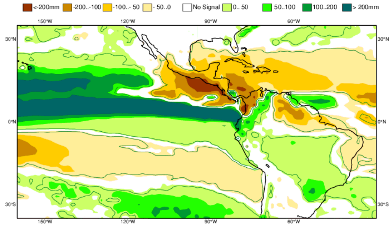
ECMWF Seasonal Forecast Mean precipitation anomaly Forecast start is 01/05/26, climate period is 1993-2016 Ensemble size = 51, climate size = 600
