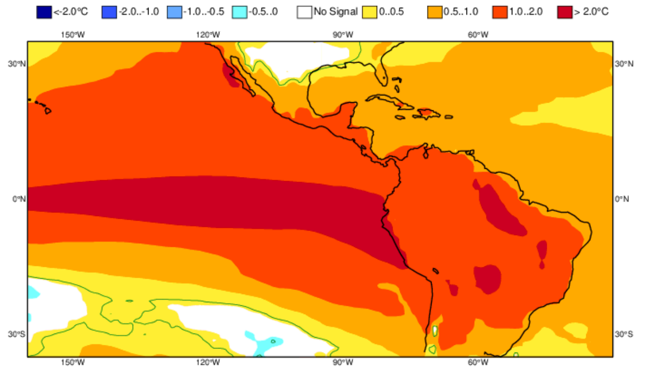
System 5 ECMWF Seasonal Forecast JJA 2026 Mean 2m temperature anomaly Shaded areas significant at 10% level Solid contour at 1% level Forecast start is 01/05/26, climate period is 1993-2016 Ensemble size = 51, climate size = 600
